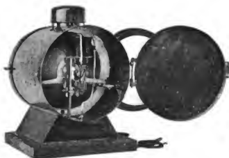
Fig. 3293. Electric Headlight. General Electric Co.
